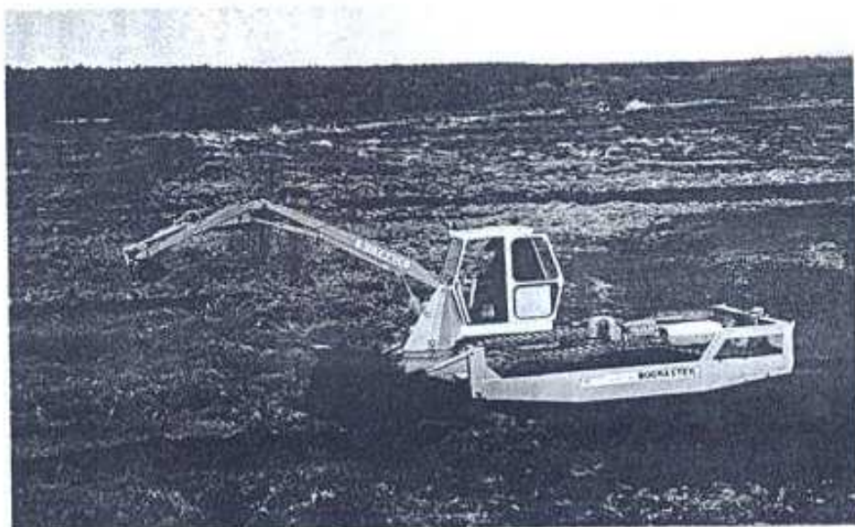
Bogmaster fitted with Big Track Screw Leveller
