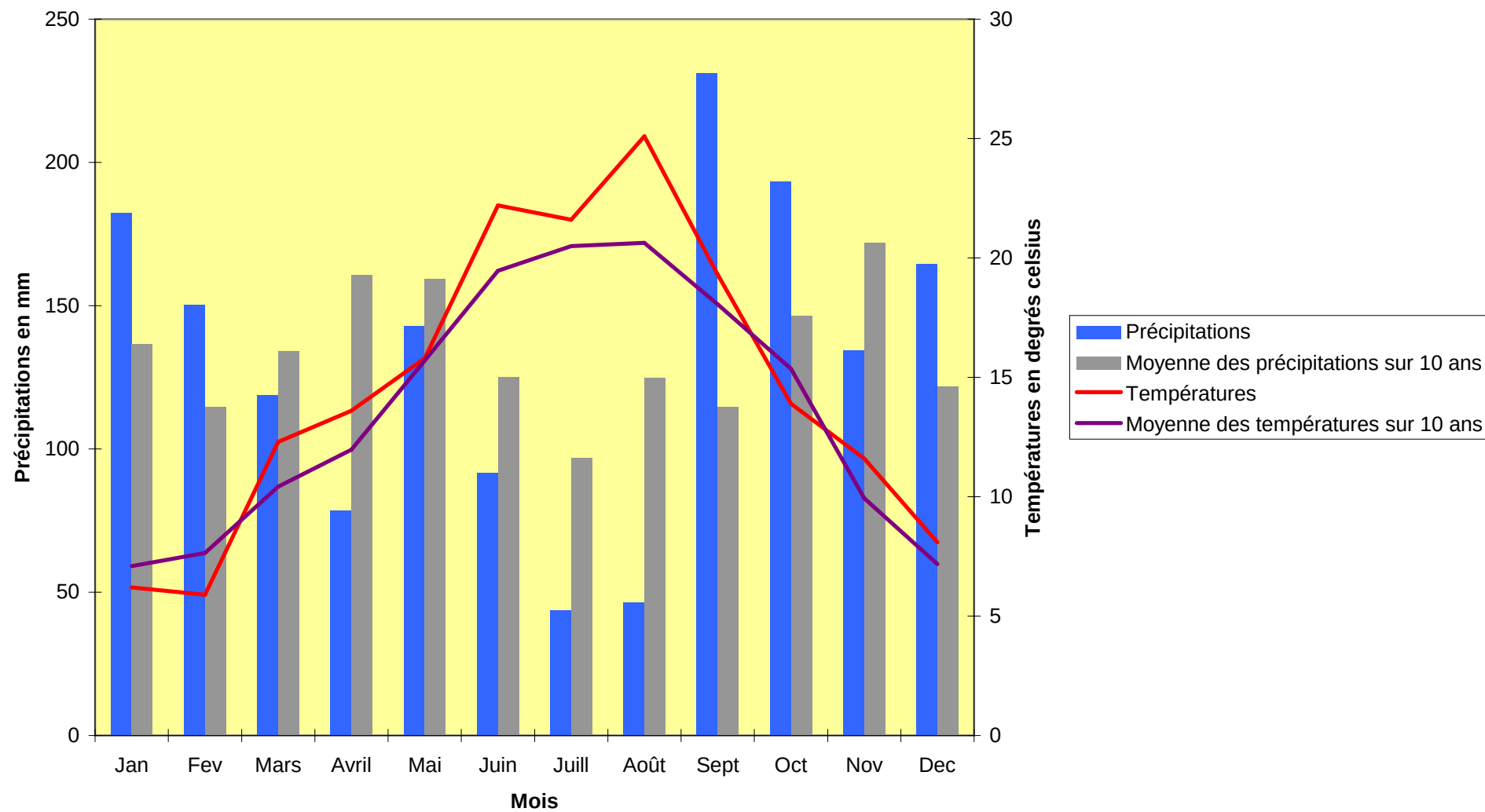
Diagramme ombrothermique Arette/Oloron 2003
